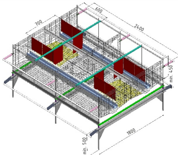
Dimensions of alternative module
