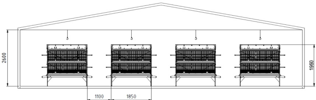
Location of technological equipment in hall
